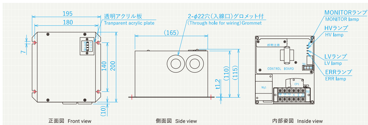
寸法図 Dimensional drawing
